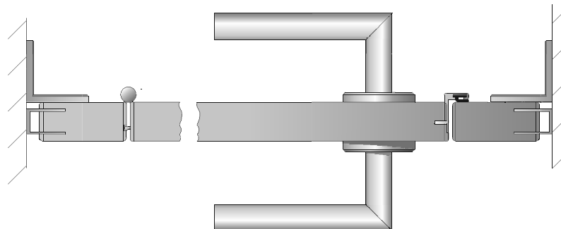
2 Cubicle front section with door handle
