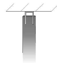
5 Wall connection with an U-profile as a shadow gap
