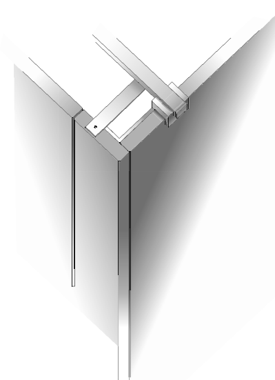
4 Corner attachment
